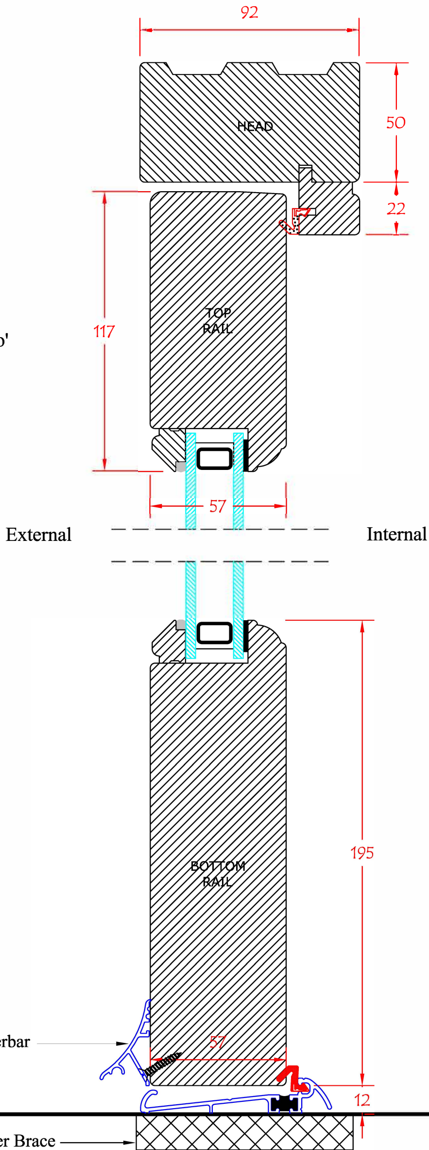
Threshold Detail 4.
