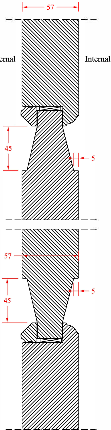
57mm Thick Raised & Fielded Panel
