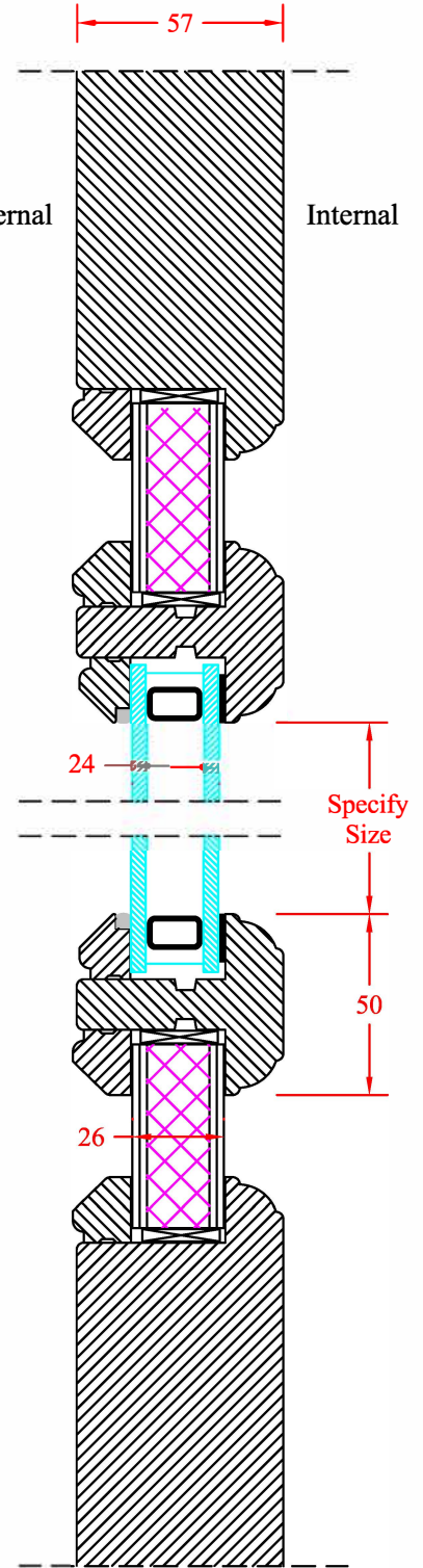
24mm Thick DGU Glazed Vision Panel
