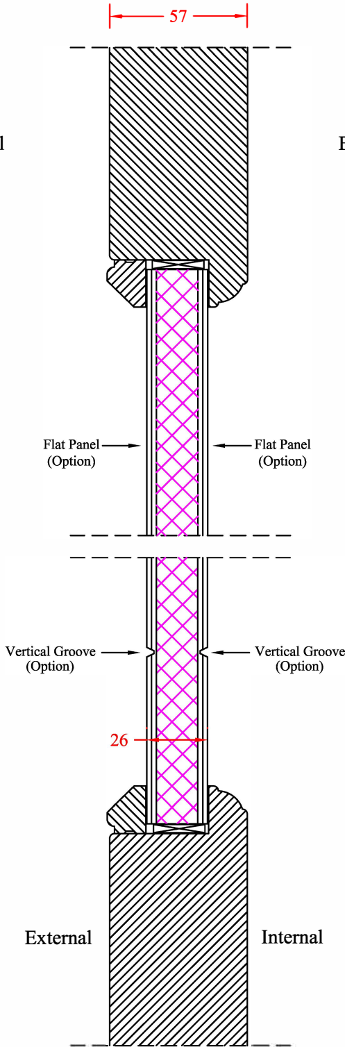
26mm Thick Insulated Panel
