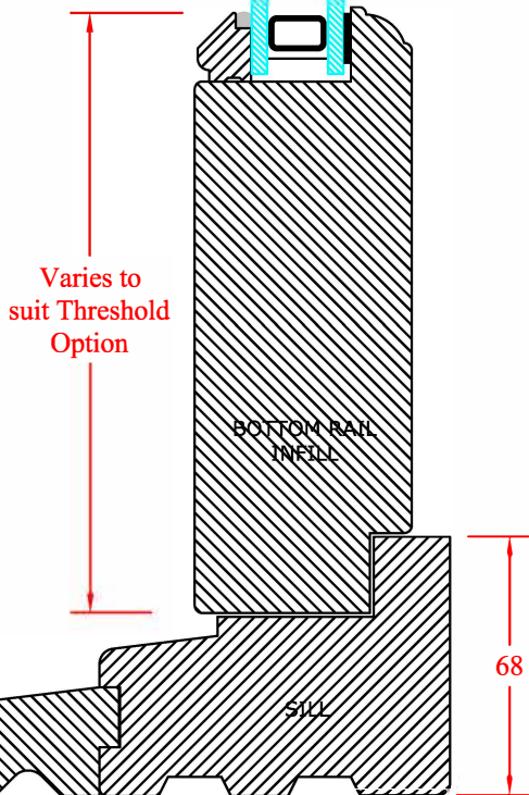
Inward Opening Profile
